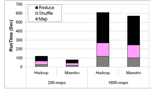
Figure 4. Sort on Grid5000: detailed performance of each stage in Maestro against native Hadoop
