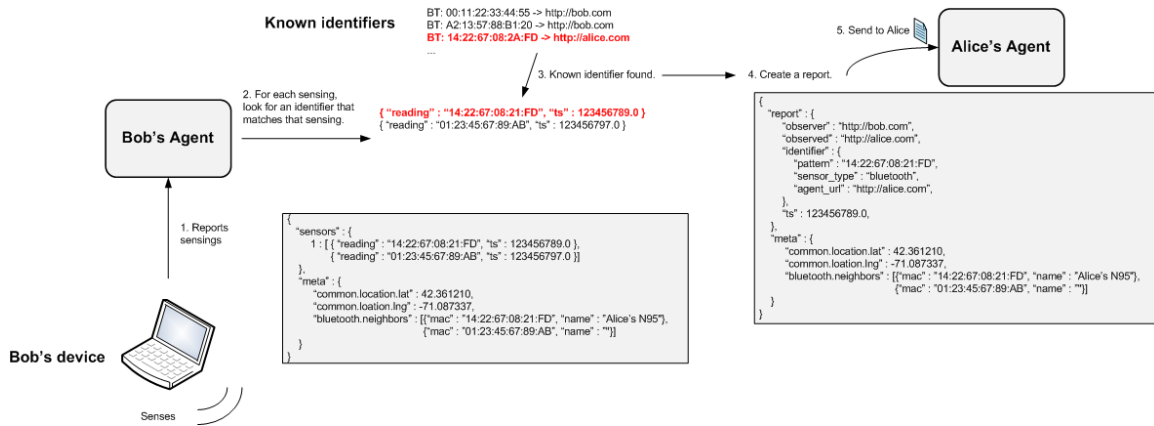
Figure 3-3: Workflow of raw contextual data being transformed into reports and shared with other agents.
