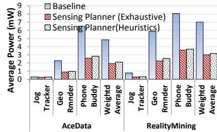
Figure 10: Energy savings by Sensing Planner
