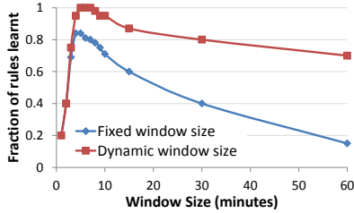
Figure 3: Effect of window size on batching
