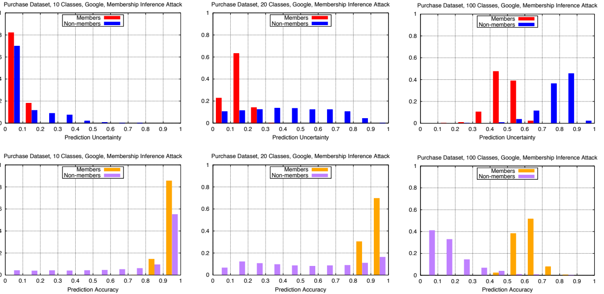
Fig. 12: Classification uncertainty (top row) and prediction accuracy (bottom row) of the target model for the members of its training dataset vs. non-members, visualized for several sample classes. The difference between the member and non-member output distributions is among the factors that our attack exploits to infer membership. The accuracy of our attack is higher for the models where the two distributions are more distinguishable (See Table II).
