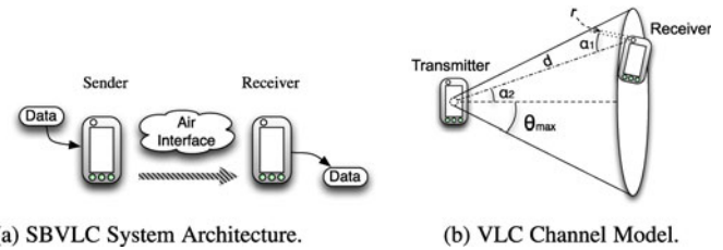
Fig. 1. SBVLC system architecture and channel model.
