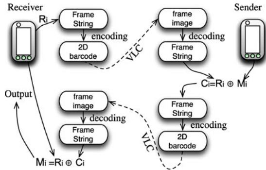
Fig. 10. Two-phase message transfer scheme.
