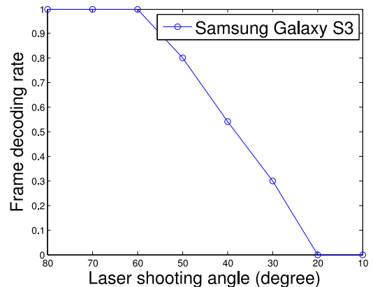
Fig. 19. Jamming experiment. (Tested on Galaxy S3.)
