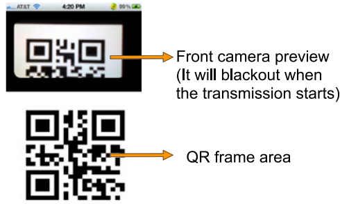
Fig. 12. User interface.
