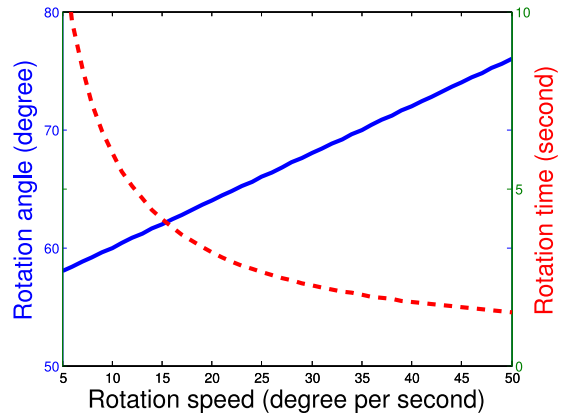
Fig. 18. Rotation angle and time trade-off.
