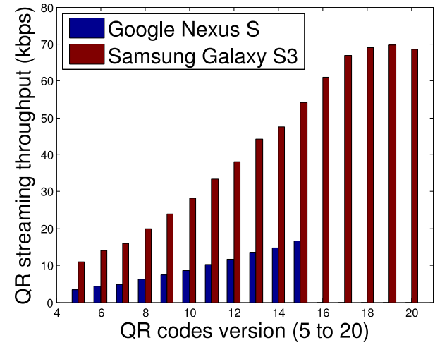
Fig. 6. Channel robustness and QR streaming throughput.
